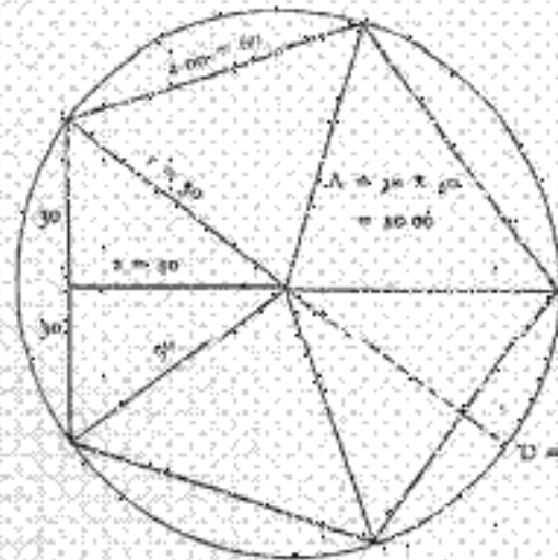
Figure 58. Derivation of the constant for calculating the area of a regular five-sided figure. Numbers in light type are decimal; numbers in bold type are sexagesimal.
